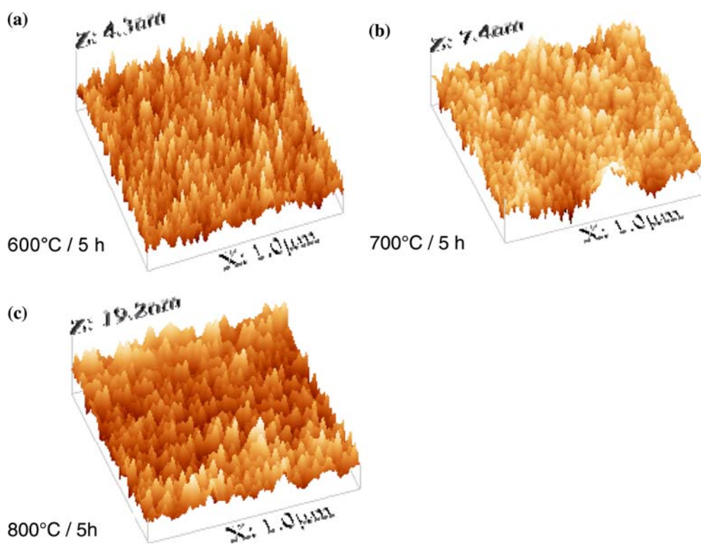
Fig. 5 Atomic Force microscopy images of \text{Fe}_2\text{Ta}_2\text{O}_8 thin films deposited on Si (100) annealed at (a) 600°C/5 h, (b) 700°C/5 h and (c) 800°C/5 h
